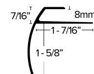
LVT 618 Stair Nosing 8MM LVT TRIM FOR STAIR NOSE IN 1-5/8" DROP. FINISH: EA, EN, BRZ
