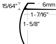
LVT 604 Stair Nosing 6MM LVT TRIM FOR STAIR NOSE IN 1-5/8" DROP. FINISH: EA, EN, BRZ
