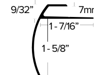
LVT 612 Stair Nosing 7MM LVT TRIM FOR STAIR NOSE IN 1-5/8" DROP. FINISH: EA, EN, BRZ
