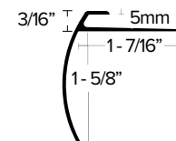
LVT 608 Stair Nosing 5MM LVT TRIM FOR STAIR NOSE IN 1-5/8" DROP. FINISH: EA, EN, BRZ, EBLK
