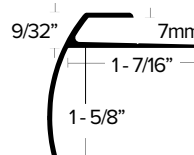
LVT 622 Stair Nosing 12MM LVT TRIM FOR STAIR NOSE IN 1-5/8" DROP. FINISH: EA, EN, BRZ, EBLK
