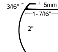
LVT 610 Stair Nosing (long) 5MM LVT TRIM FOR STAIR NOSE IN 2" DROP. FINISH: EA, EN, BRZ
